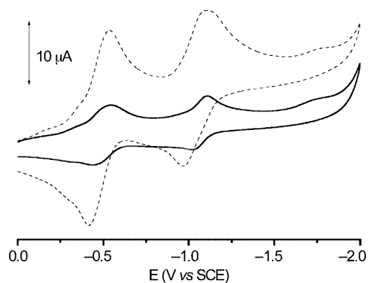
Figure 3. Cyclic voltammogram of tris(quinones) 20 (---) and 21 (—) (room temperature, in \text{CH}_2\text{Cl}_2 solutions containing 0.1 M \text{TBAPF}_6 as a supporting electrolyte; scan rate = 100 \text{ mV}\cdot\text{s}^{-1} ).
