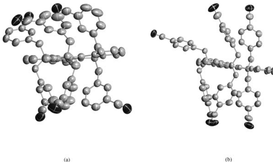
Figure 1. X-ray diffraction structures of nitriles 5e (a) and 5f (b).
